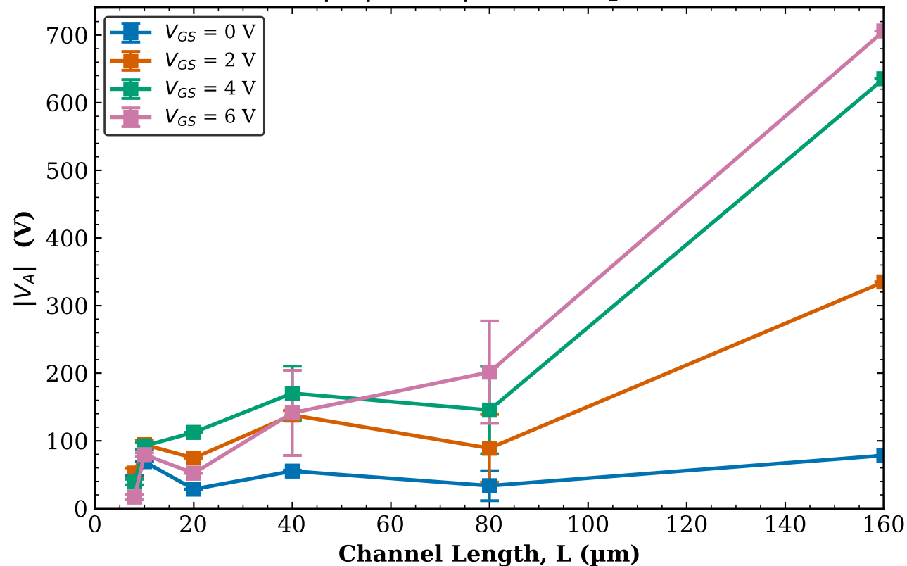
TFT1 Combined (Tr. 1 & 2) |V_A| vs L | W = 50\text{ }\mu\text{m}
